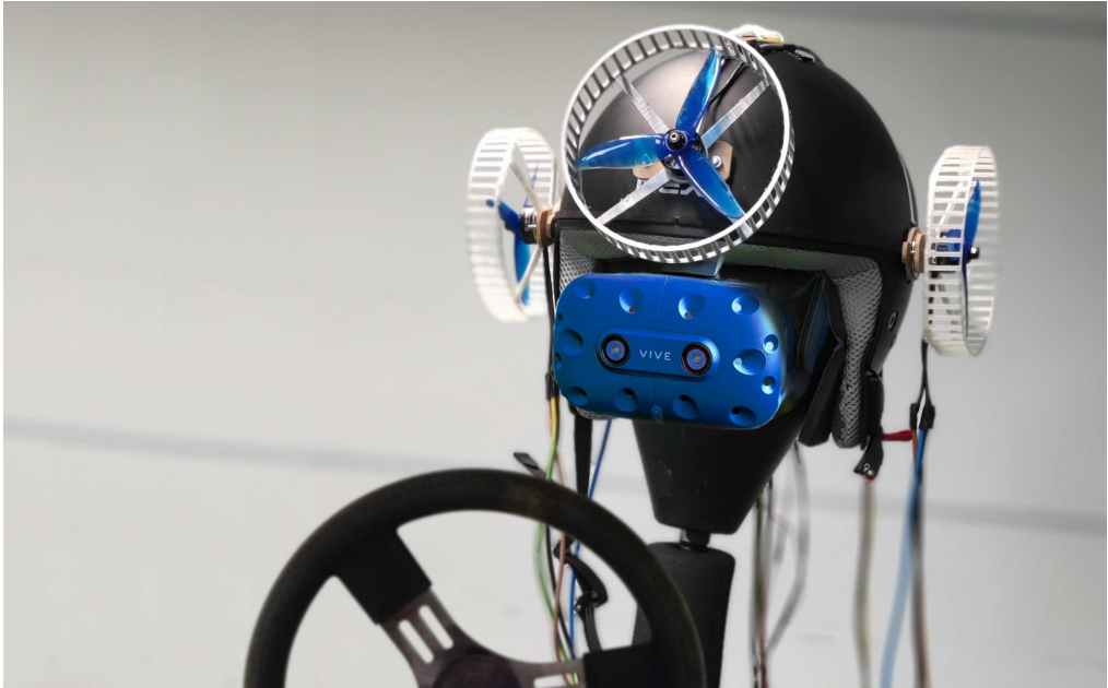
Fig. 1. We envision Odin's Helmet to enable the perception of g-forces in Virtual Reality. Our head-worn prototype has four propellers attached that actuate the direction of the user's head. Our vision is that the displacement, combined with the otolith organ and visual stimuli, simulate the perception of g-forces and self-motion in the virtual world.
