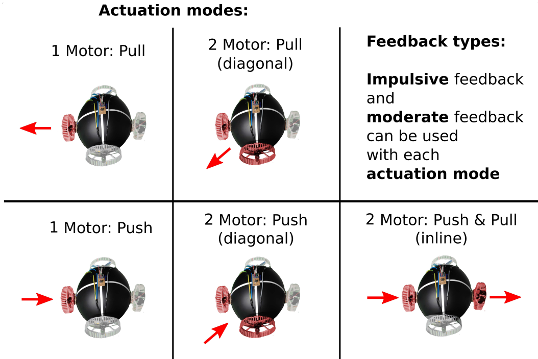
Fig. 4. Odin's Helmet offers two Feedback types: impulsive and moderate and 5 actuation types: Push forces the user's head to be pushed into a direction, while Pull redirects the user's head through pulling. Push (diagonal) and Pull (diagonal) use two adjacent propellers respectively. Push & Pull (inline) uses one propeller on each side.
