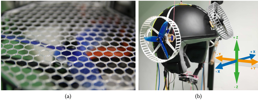
Fig. 5. (a) : A 3D-printed safety net is attached to the propeller case to ensure user safety. If desired, a tighter net can also serve as a mechanical barrier to limit the maximum generated force by restricting airflow. (b) : Testbed for Odin's Helmet for early evaluation. The helmet is hung on the ceiling and spring feathers are used to measure force in Newton. An accelerator was attached at the top of the helmet to measure acceleration. Phonometers are placed inside the helmet and in one-meter distance to measure the produced sound levels.
